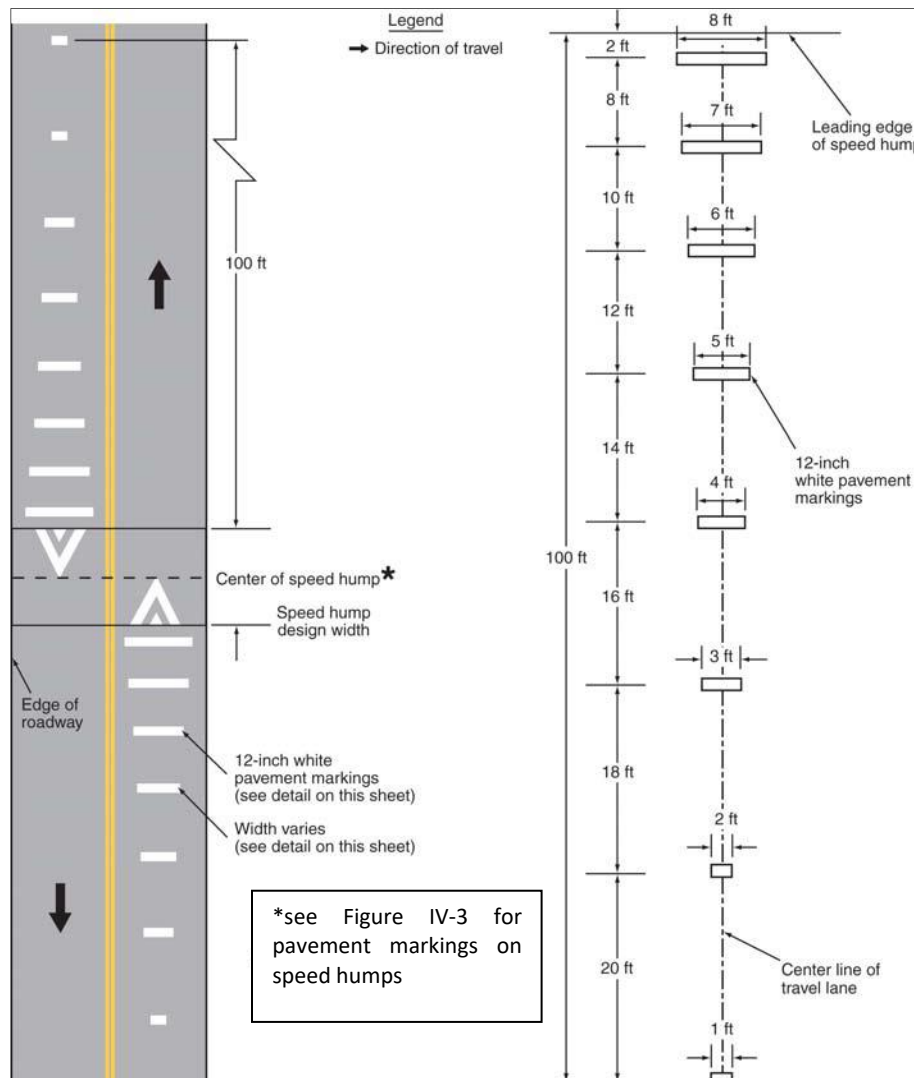
SPEED HUMPS ADVANCE WARNING MARKINGS
