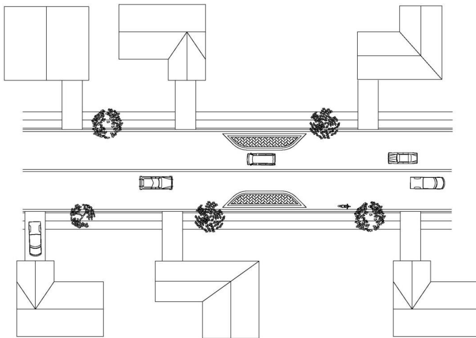
DIAGRAM OF CHOKER- FIGURE III-9
