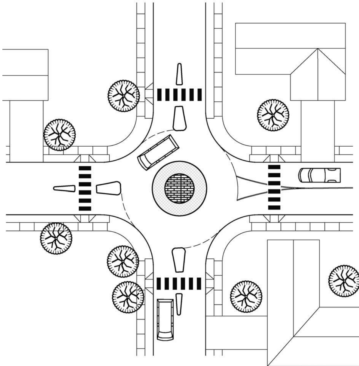
DIAGRAM OF A MINI ROUNDABOUT FIGURE III-22
